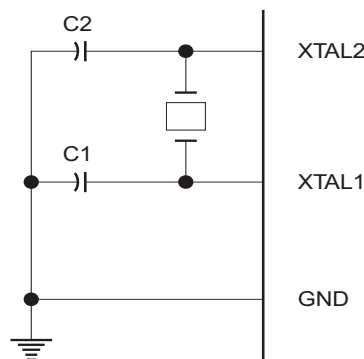
Figure 1. Oscillator Connections
