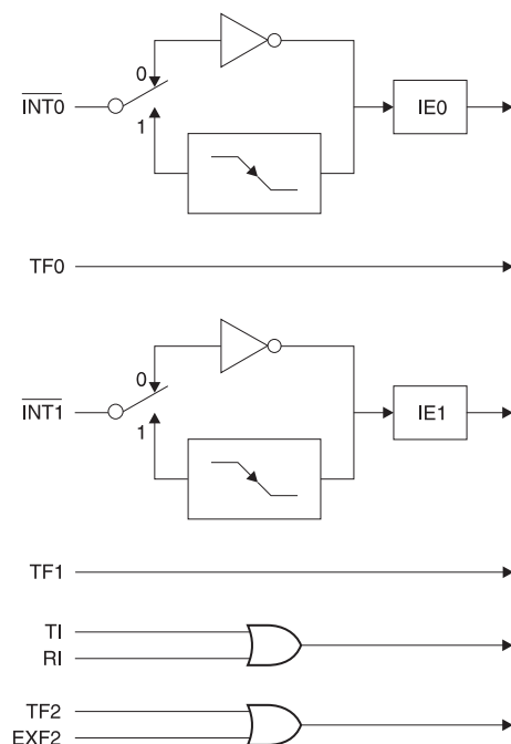
Figure 6. Interrupt Sources
