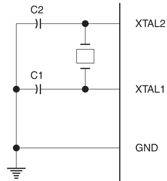
Figure 7. Oscillator Connections
